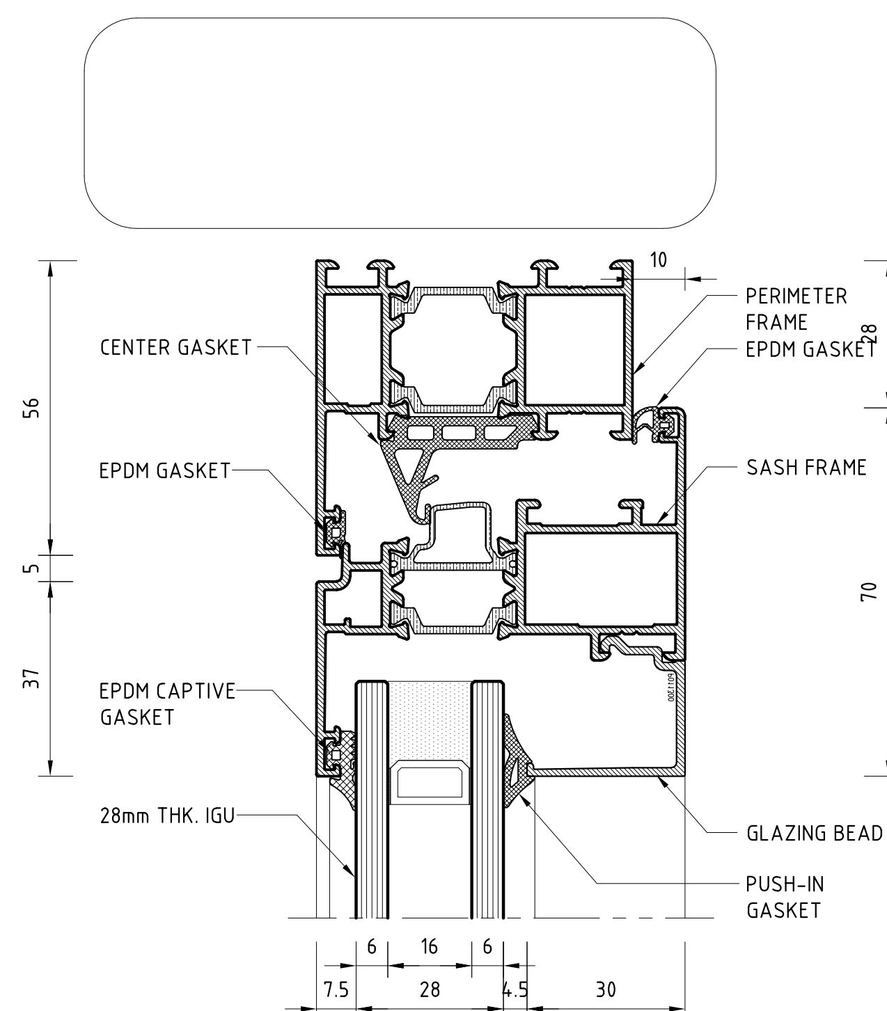
HEAD DETAIL
