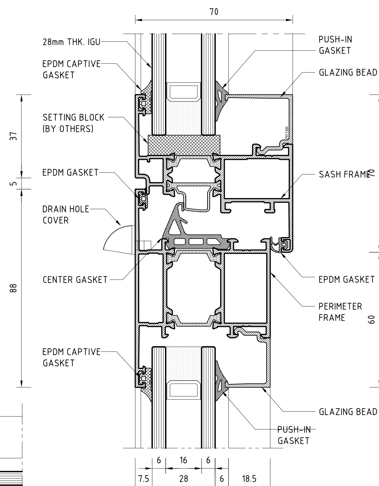
HORIZONTAL FRAME DETAIL
