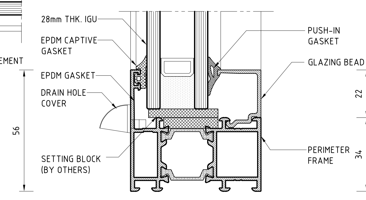
HORIZONTAL FRAME DETAIL
